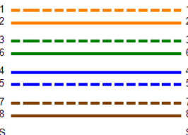
Wire Map (T568B) PASS
