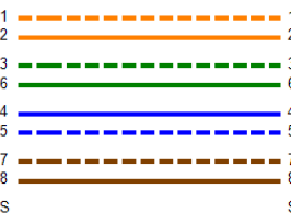
Wire Map (T568B)
